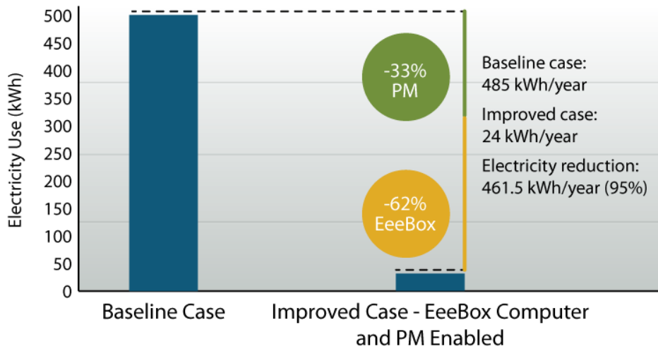
Figure 4. Mini Computer + Power Management = 95% Savings
